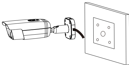
Side wiring
